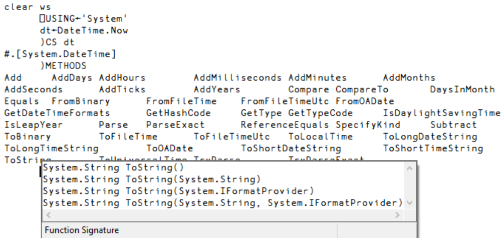
Figure 3-2: Function signature – multiple arguments
