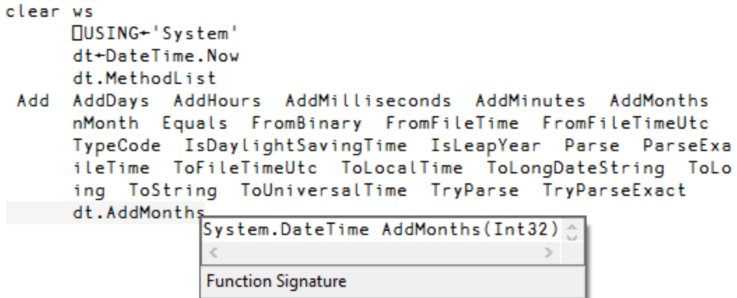
Figure 3-1: Function signature – single integer argument
